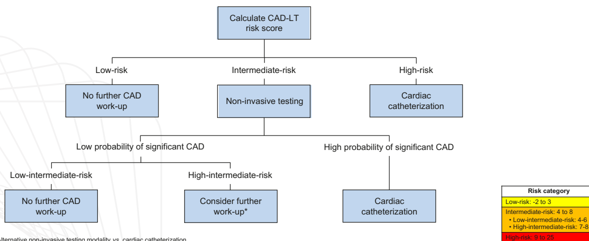
Fig.2 CAD-LT algorithm
