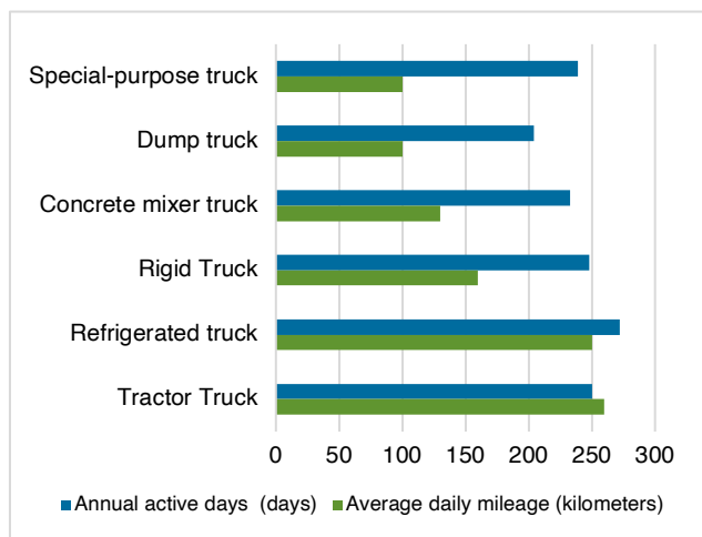
Figure 5. Annual active days and daily mileage of major operational trucks in Shenzhen (Source: NEICV)
