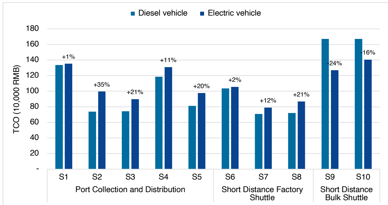
Figure 14. 5-year TCO comparison of diesel and electric vehicles
