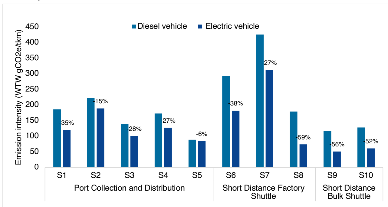
Figure 15. Well-to-wheel greenhouse gas emission intensity comparison for diesel and electric vehicles
